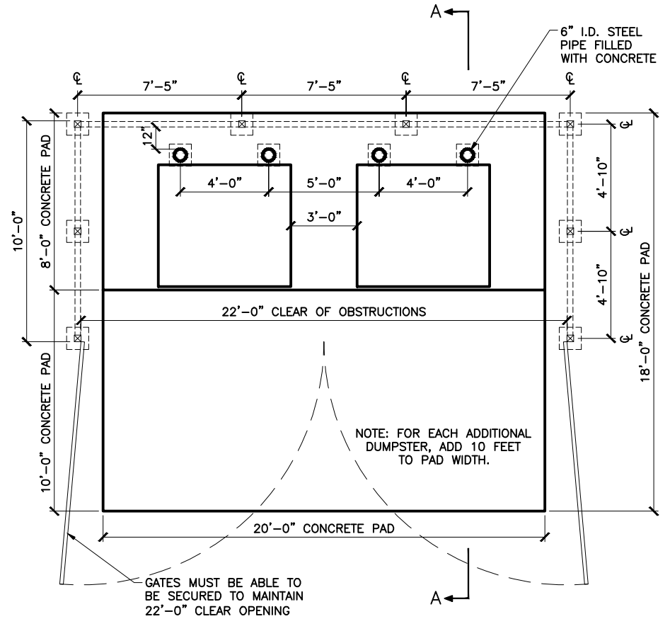
PLAN
