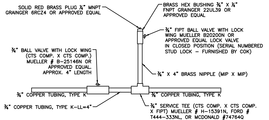
ELEVATION VIEW NOT TO SCALE
