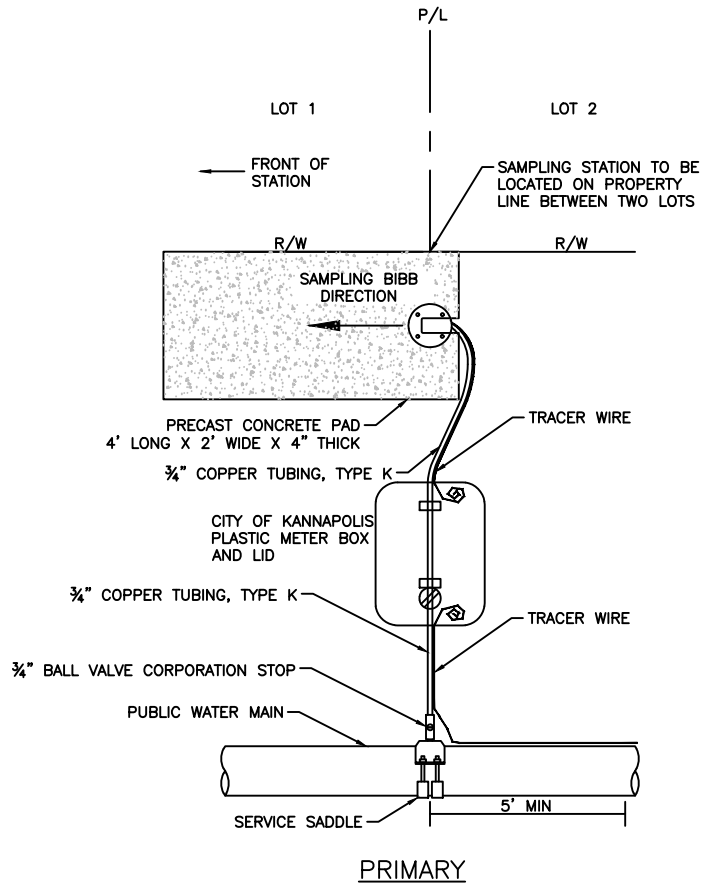
PLAN VIEW NOT TO SCALE
