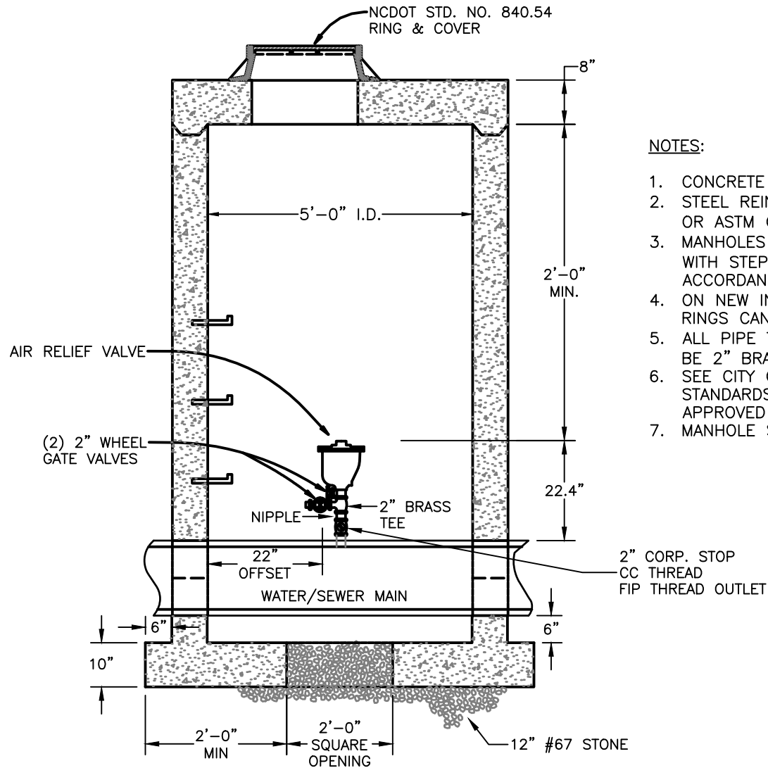
SECTION THROUGH MANHOLE
