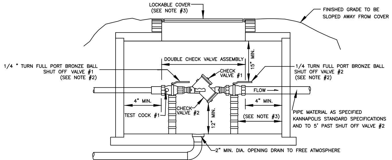
ELEVATION VIEW
