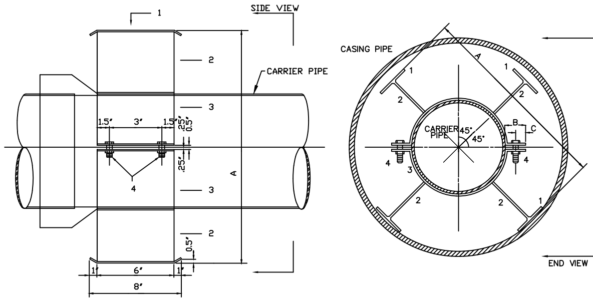
LEGS ROTATED OUT OF POSITION FOR CLARITY
