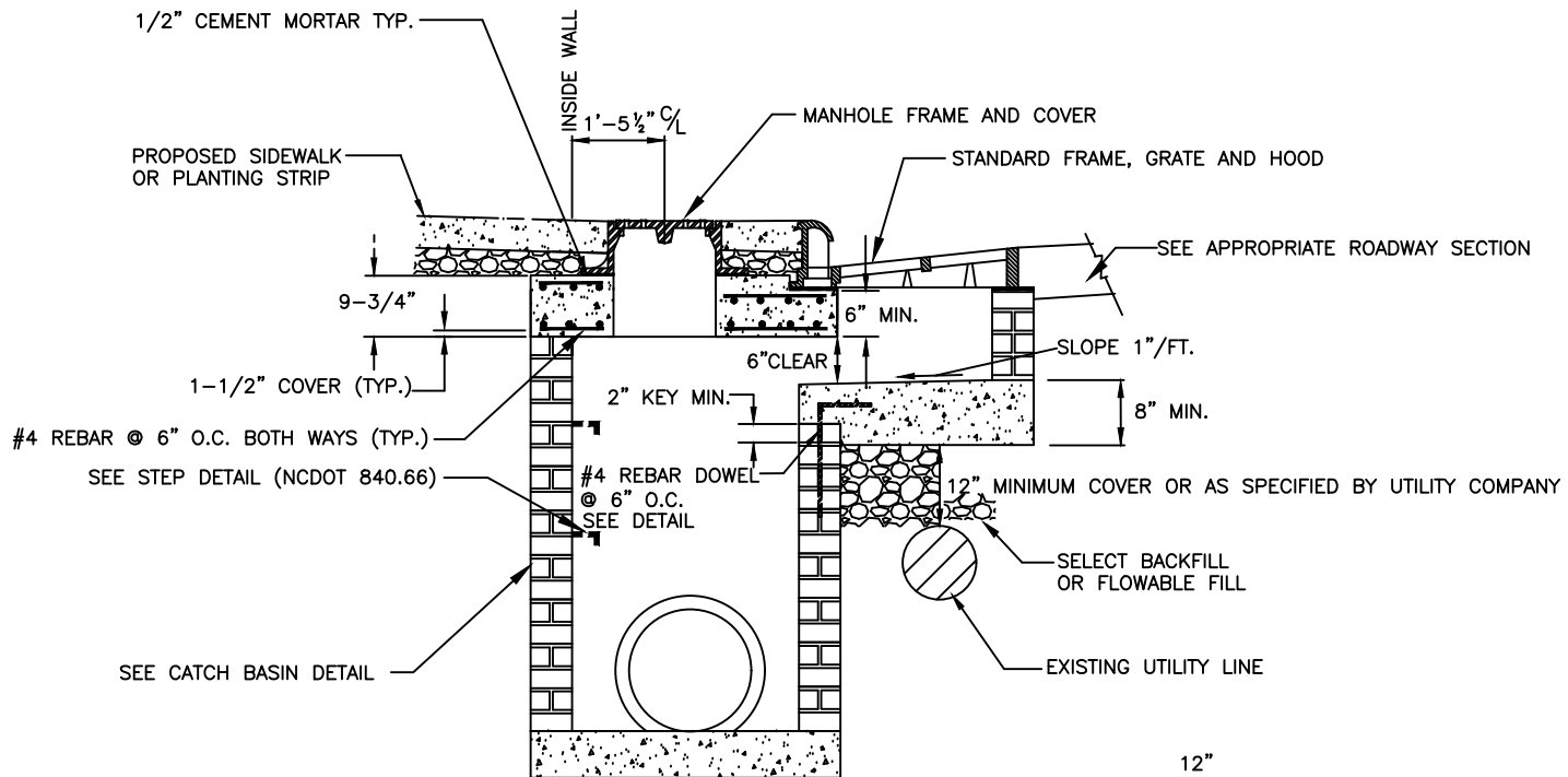
OFFSET CATCH BASIN EXISTING UTILITY CONFLICT
